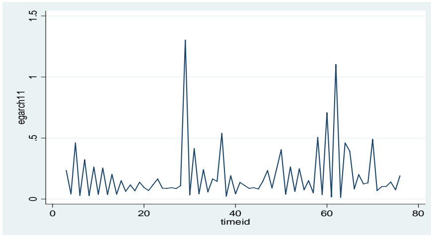
egarch11
