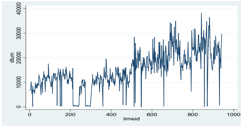
dturn
